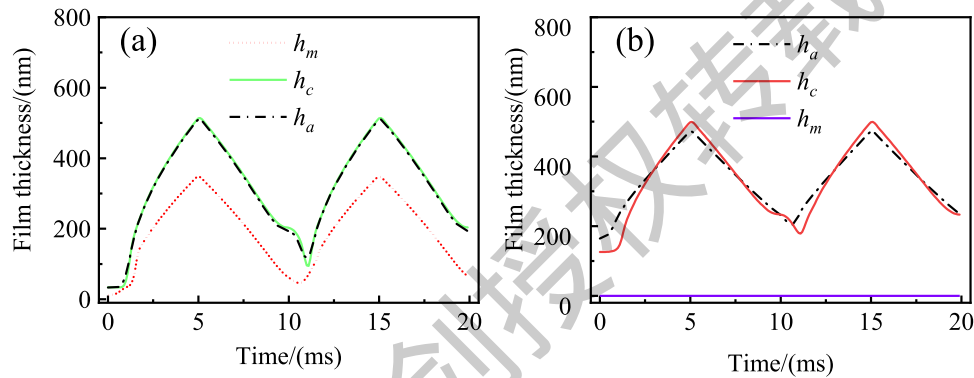
Fig. 16. The variation of film thickness during start up and shut down process. (a) Smooth surface (b) Rough surface.
