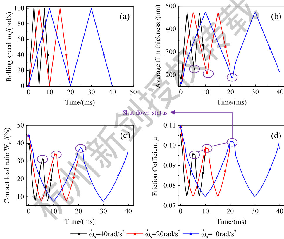
Fig. 19. Effects of angular acceleration on the lubrication during the start up and shut down process.
