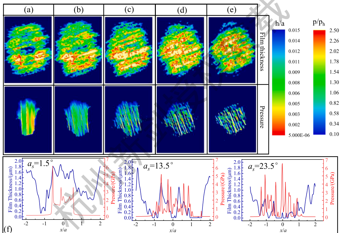
Fig. 8. Film thickness and pressure for different helix angle (Rough, \omega_s = 40\text{rad/s} ). (a) \alpha_s = 1.5 deg (b) \alpha_s = 7.5 deg (c) \alpha_s = 13.5 deg (d) \alpha_s = 19.5 deg (e) \alpha_s = 23.5 deg and (f) film thickness and pressure in the X rolling direction.
