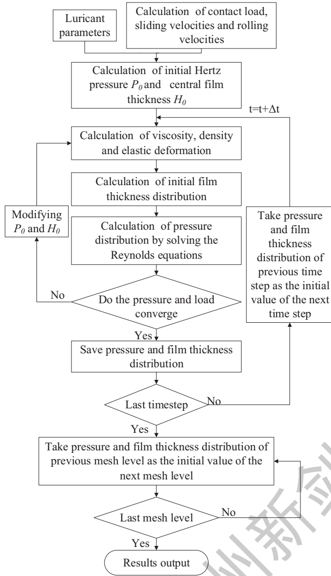
Fig. 4. Flowchart of transient EHL in PRSM.
