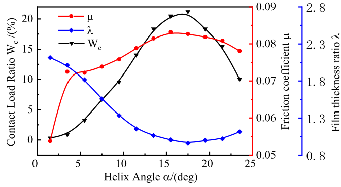
Fig. 9. Effect of helix angle on the film thickness ratio, contact load ratio and coefficient of friction.
