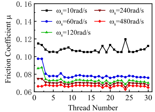
Fig. 11. Friction distribution in different screw speed.
