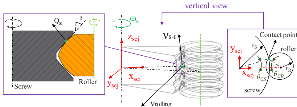
Fig. 2. The contact geometry of the roller and screw.
