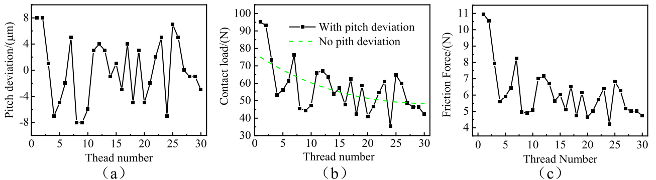
Fig. 10. Pith deviations (a), load distribution (b), friction distribution (c) of all threads.
