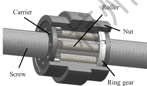
Fig. 1. Planetary roller screw mechanism.
