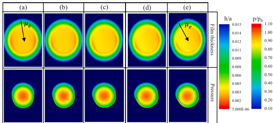
Fig. 7. Film thickness and pressure contours for different helix angle (Smooth, \omega_s = 40\text{rad/s} ). (a) \alpha_s = 1.5 deg (b) \alpha_s = 7.5 deg (c) \alpha_s = 13.5 deg (d) \alpha_s = 19.5 deg and (e) \alpha_s = 23.5 deg.
