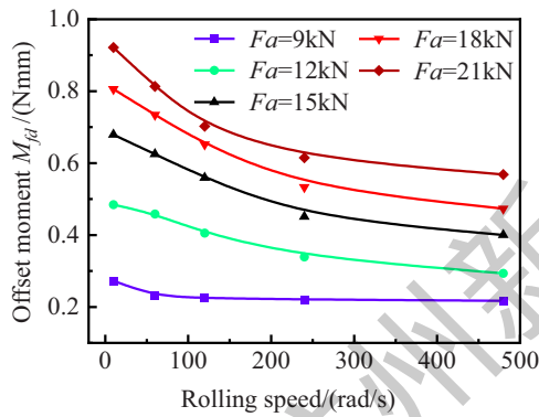
Fig. 13. Dynamic friction offset moment under different rolling speed and axial force.
