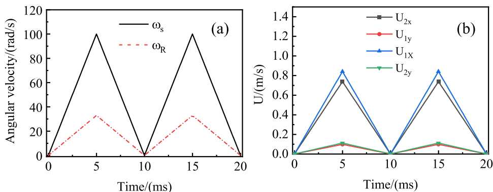
Fig. 14. Angular velocity of roller revolution and screw rotation (a) and entraining velocity (b) during start up and shut down process.
