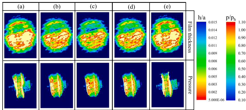
Fig. 18. Film thickness and pressure contours during start up and shut down process (Rough). (a) t = 11 ms (b) t = 13 ms (c) t = 15 ms (d) t = 17 ms and (e) t = 20 ms.
