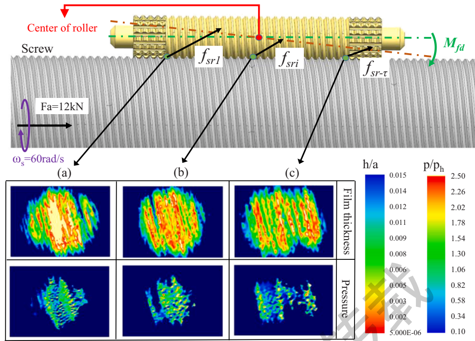
Fig. 12. The dynamic friction offset torque of single roller. (a) Lubrication performance of thread 1 (b) Lubrication performance of thread 12 and (c) Lubrication performance of thread 30.
