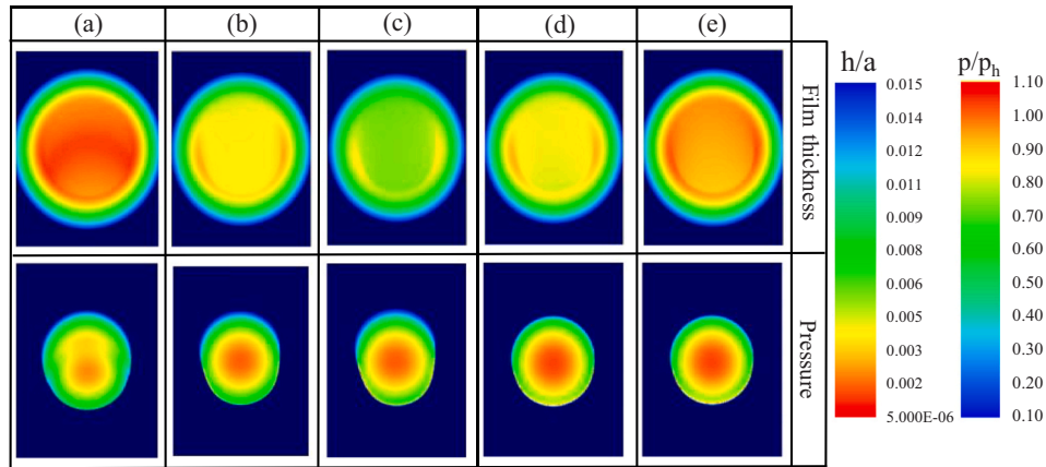
Fig. 15. Film thickness and pressure contours during the start up and shut down process (Smooth). (a) t = 11 ms (b) t = 13 ms (c) t = 15 ms (d) t = 17 ms and (e) t = 20 ms.
