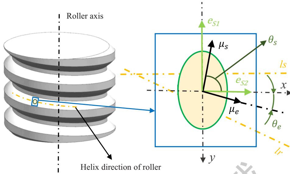
Fig. 3. The direction of sliding and entraining vector in the roller-screw interface.
